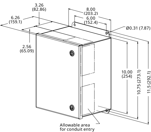
125 kA metal enclosure with lugs
