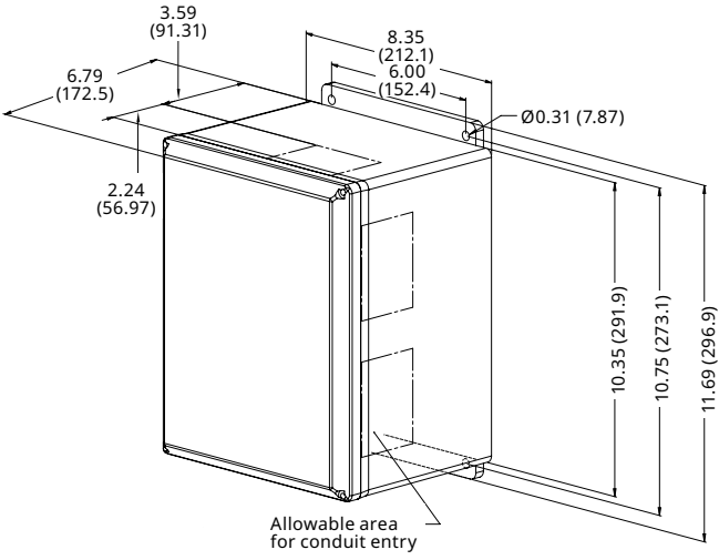
125 kA polycarbonate enclosure with lugs
