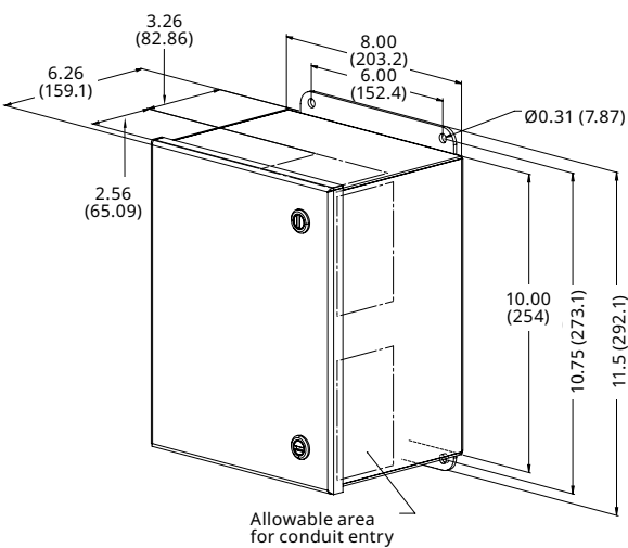
200 kA metal enclosure with lugs
