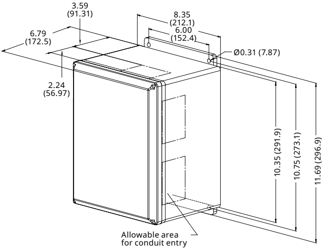
200 kA polycarbonate enclosure with lugs
